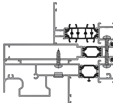
CP 130 MONORAIL + CS 86-HI (WITH CONNECTION PROFILE)
